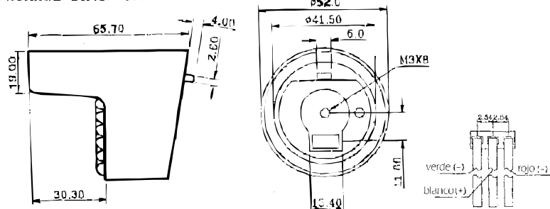
PACKAGE DIMENSIONS
