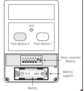
Enclosure opened, with front cover.
