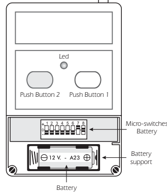
Enclosure opened, with front cover.
